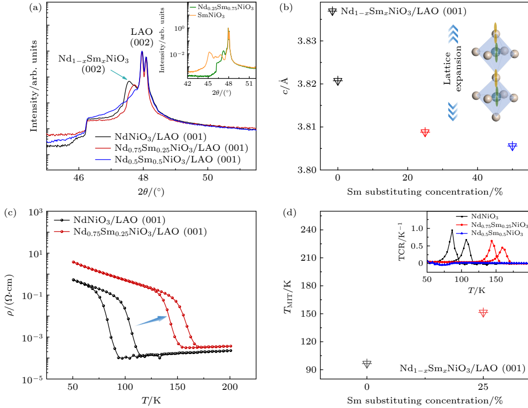
图4 \text{Nd}_{1-x}\text{Sm}_x\text{NiO}_3 薄膜的晶体结构和电子相变特性 (a) \text{Nd}_{1-x}\text{Sm}_x\text{NiO}_3 ( x = 0, 0.25, 0.5 ) 薄膜的XRD图谱, 插图是 \text{Nd}_{1-x}\text{Sm}_x\text{NiO}_3 ( x = 0.75, 1 ) 薄膜的XRD图谱; (b) \text{Nd}_{1-x}\text{Sm}_x\text{NiO}_3 ( x = 0, 0.25, 0.5 ) 薄膜 c 轴晶格参数随 A 位 Sm 元素共占据比例的变化关系图; (c) \text{Nd}_{1-x}\text{Sm}_x\text{NiO}_3 ( x = 0, 0.25 ) 薄膜的阻温特性曲线; (d) \text{Nd}_{1-x}\text{Sm}_x\text{NiO}_3 ( x = 0, 0.25 ) 薄膜的相变温度随 A 位 Sm 元素共占据比例的变化关系图, 插图是 \text{Nd}_{1-x}\text{Sm}_x\text{NiO}_3 ( x = 0, 0.25, 0.5 ) 薄膜的TCR- T 曲线
