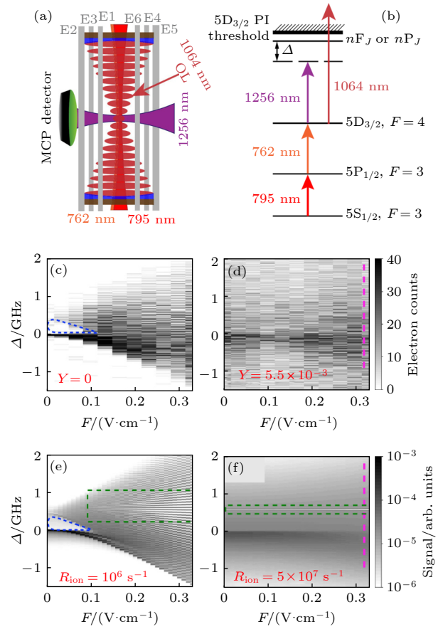
图 9 冷离子源中电场分布测量 [41] (a) 实验装置示意图; (b) ^{85}\text{Rb} 能级示意图及光电离和激发所需的激光波长; (c) 低离子计数率和 (d) 高离子计数率条件下, 实验测量的 57\text{F}_{5/2} 的 Stark 图; (e), (f) 对应的模拟 Stark 图 Fig. 9. Measurement of electric field in a cold ion source [41] : (a) Sketch of the experimental setup; (b) diagram of the utilized ^{85}\text{Rb} energy levels and configuration of laser beams for photoionization and excitation; (c), (d) experimental Stark maps of 57\text{F}_{5/2} and the neighboring hydrogenic states at the different \gamma values; (e), (f) the corresponding simulated Stark maps with empirically determined ion rates.
