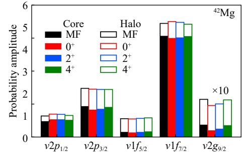
Fig. 5 Probability amplitudes of p -, f -, and g -wave components contributed to the halo and core of the MF ground state and each collective state for ^{42}\text{Mg} [48] . The probability amplitude of v2g_{9/2} is multiplied by 10. (color online)
